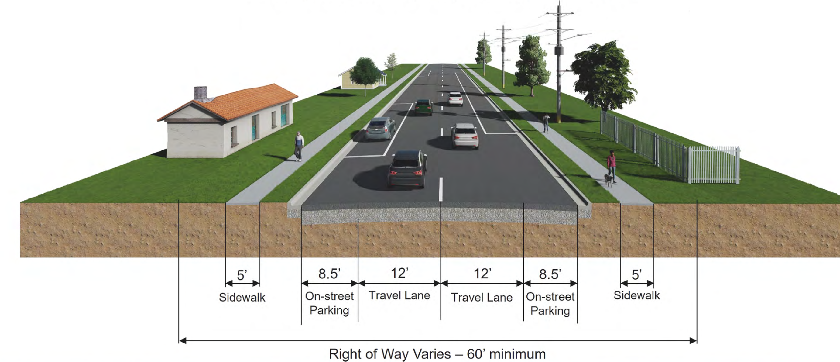
SR 24 (Waldo Road) Proposed Typical Section
